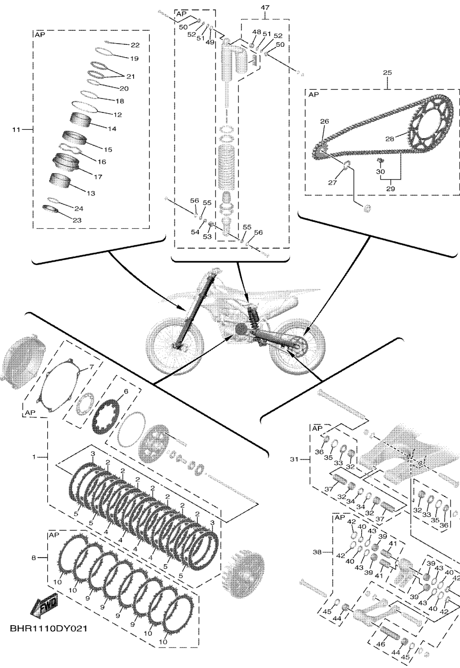
FIG. 2 MAINTENANCE PARTS KIT
